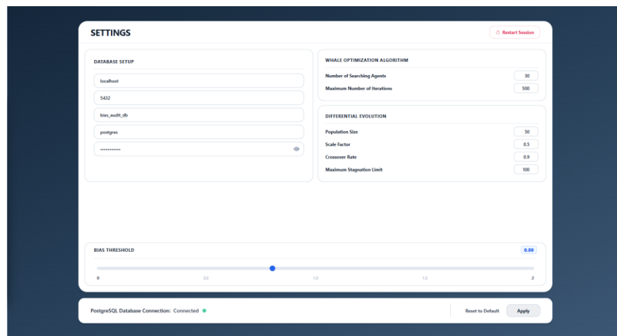
Figure 10: Settings page
