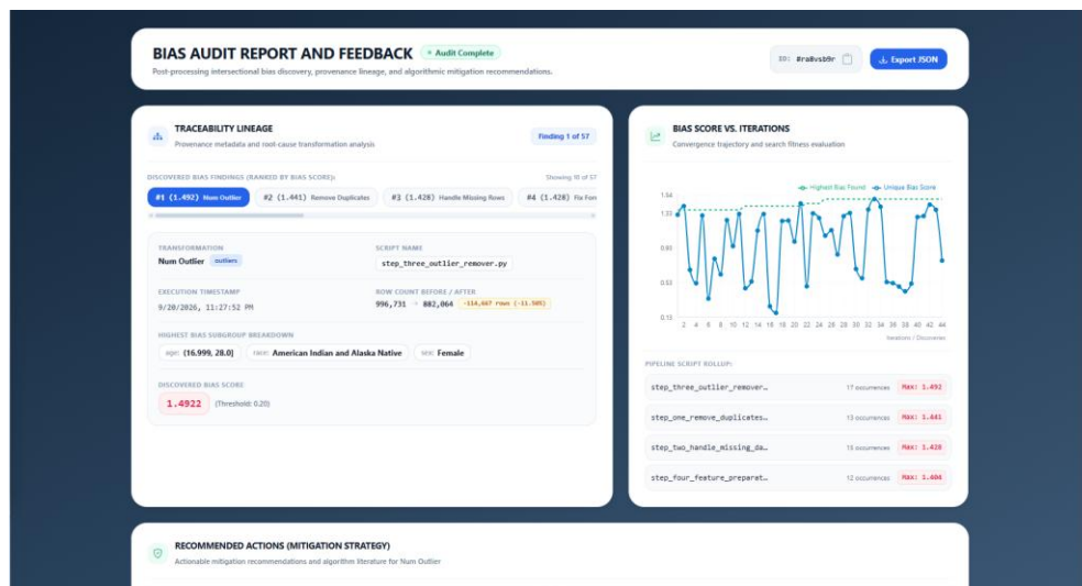
Figure 9: Results Panel
